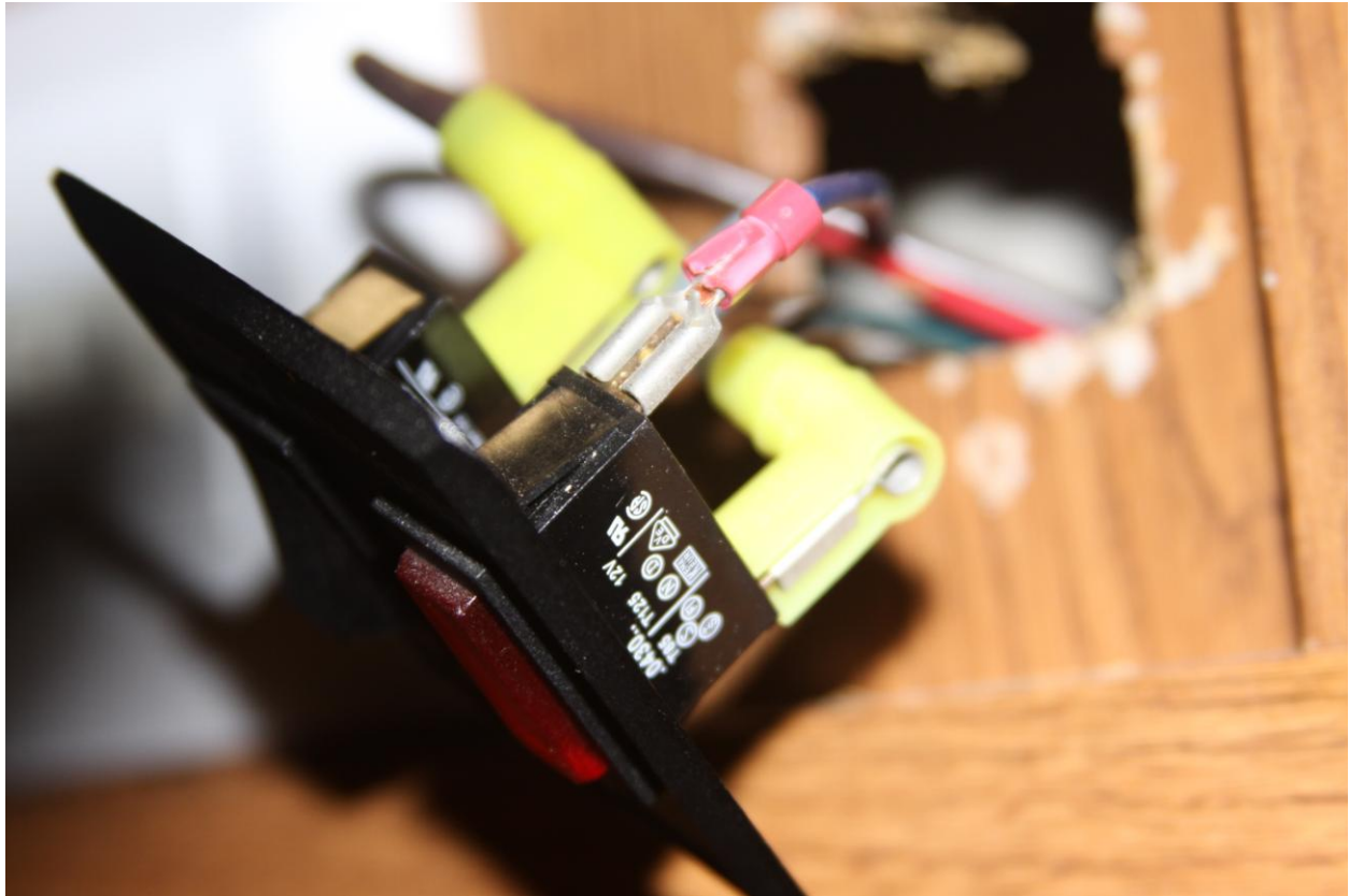
This the LED side of my switch with the switch in the position that it was mounted in.
